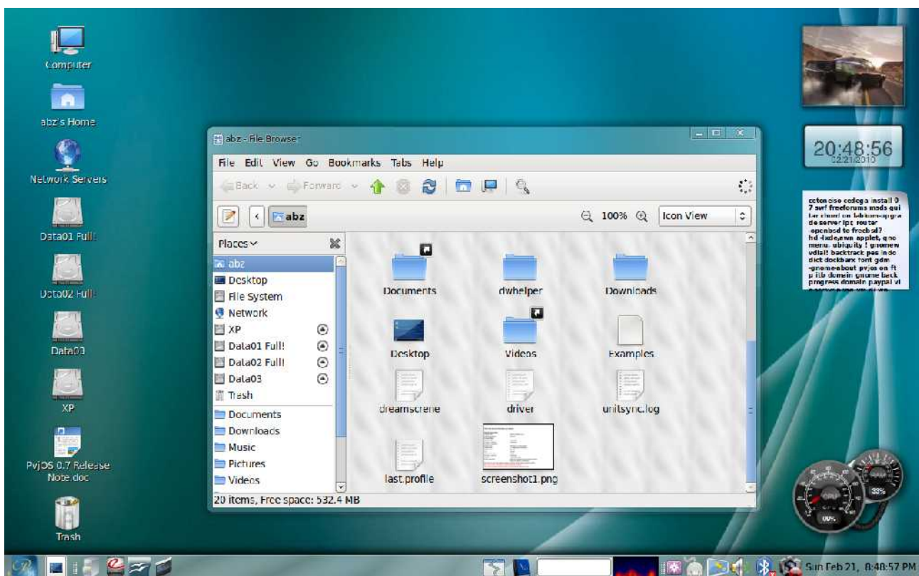
Desktop Screenshot
